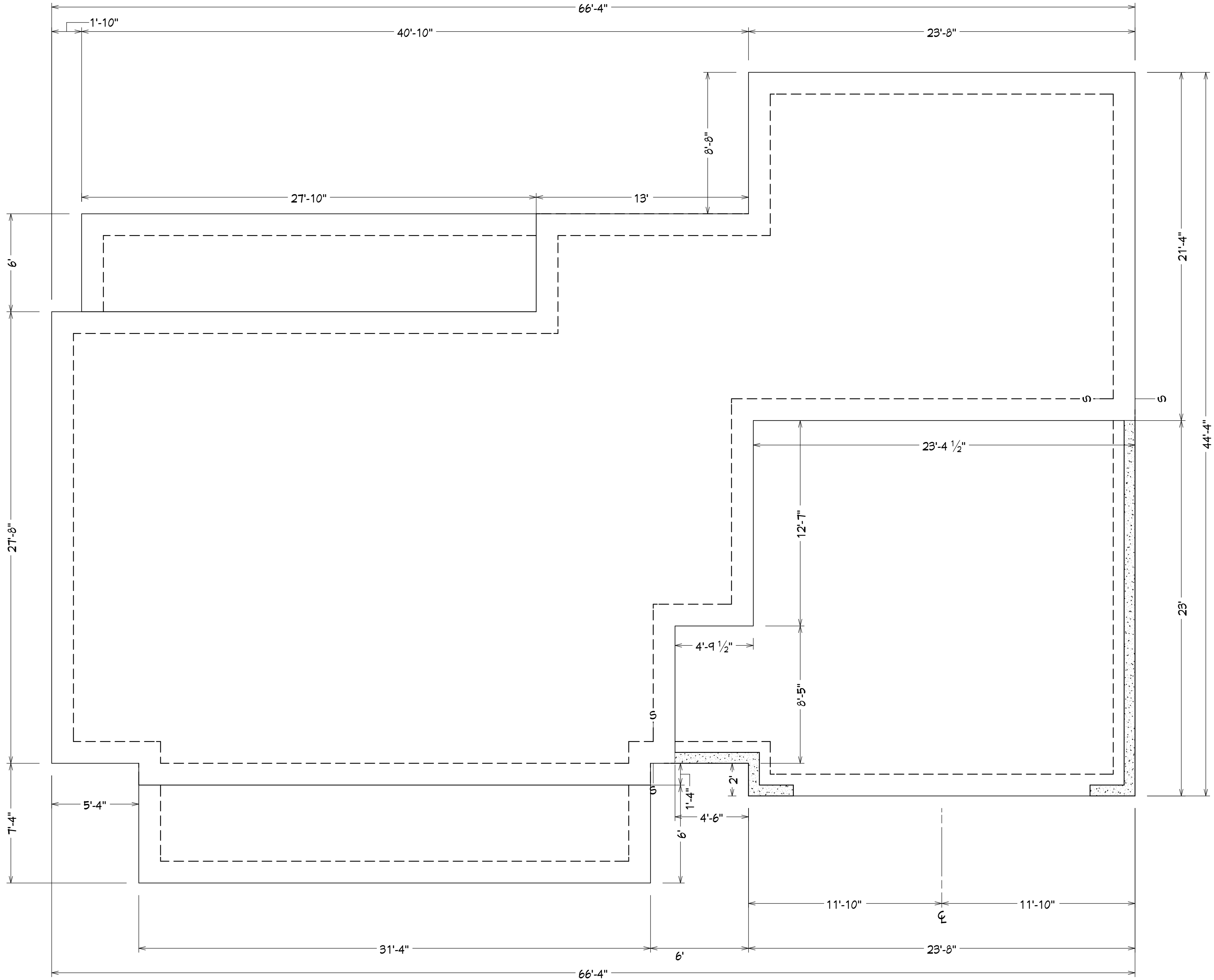
FOUNDATION 1/4 IN = 1 FT
