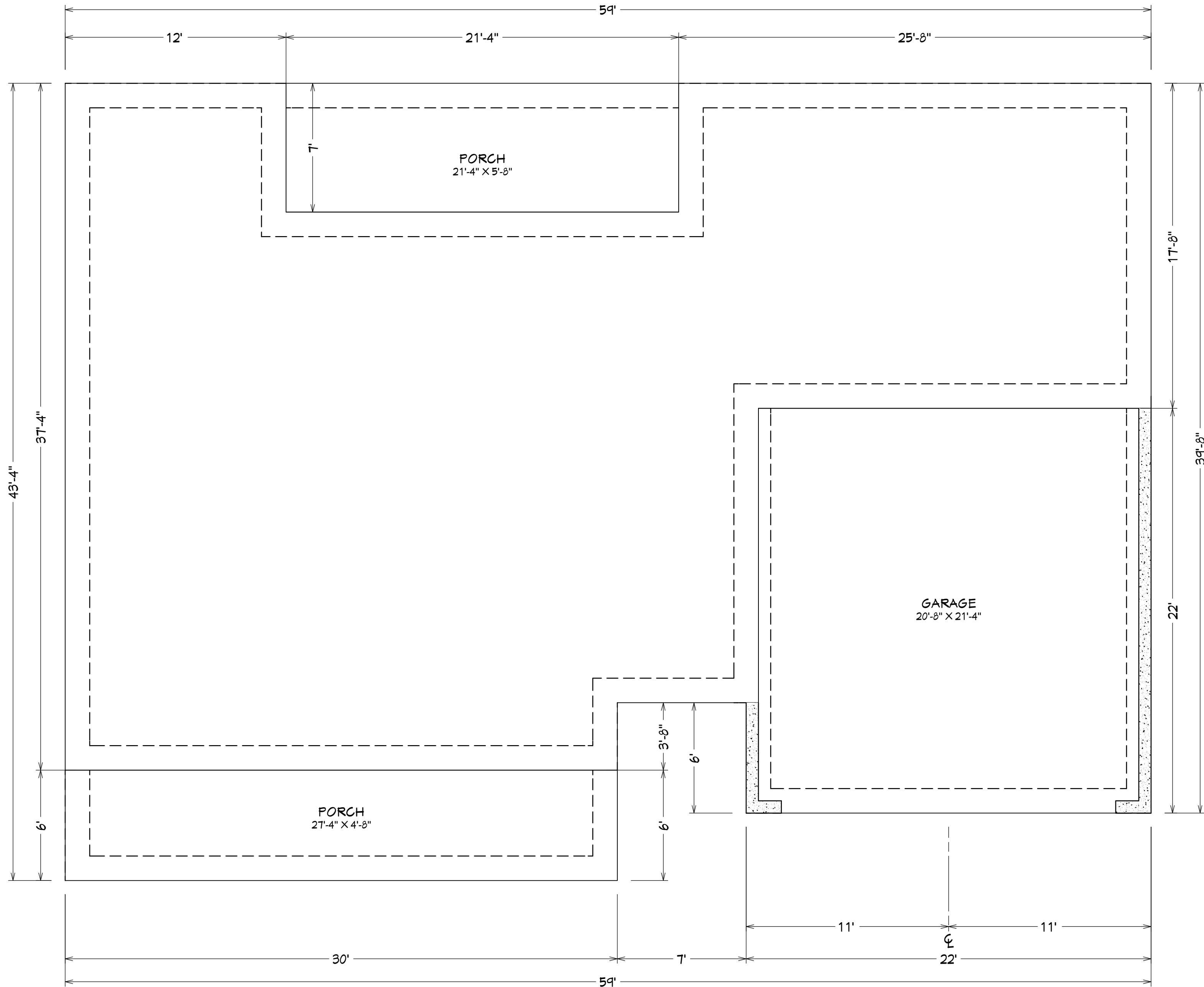
FOUNDATION 1/4 IN = 1 FT
