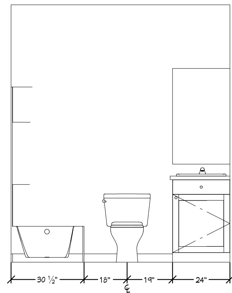
E5 ELEVATION 3 1/2 IN = 1 FT
