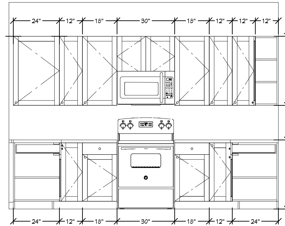
E7 ELEVATION 5 1/2 IN = 1 FT
