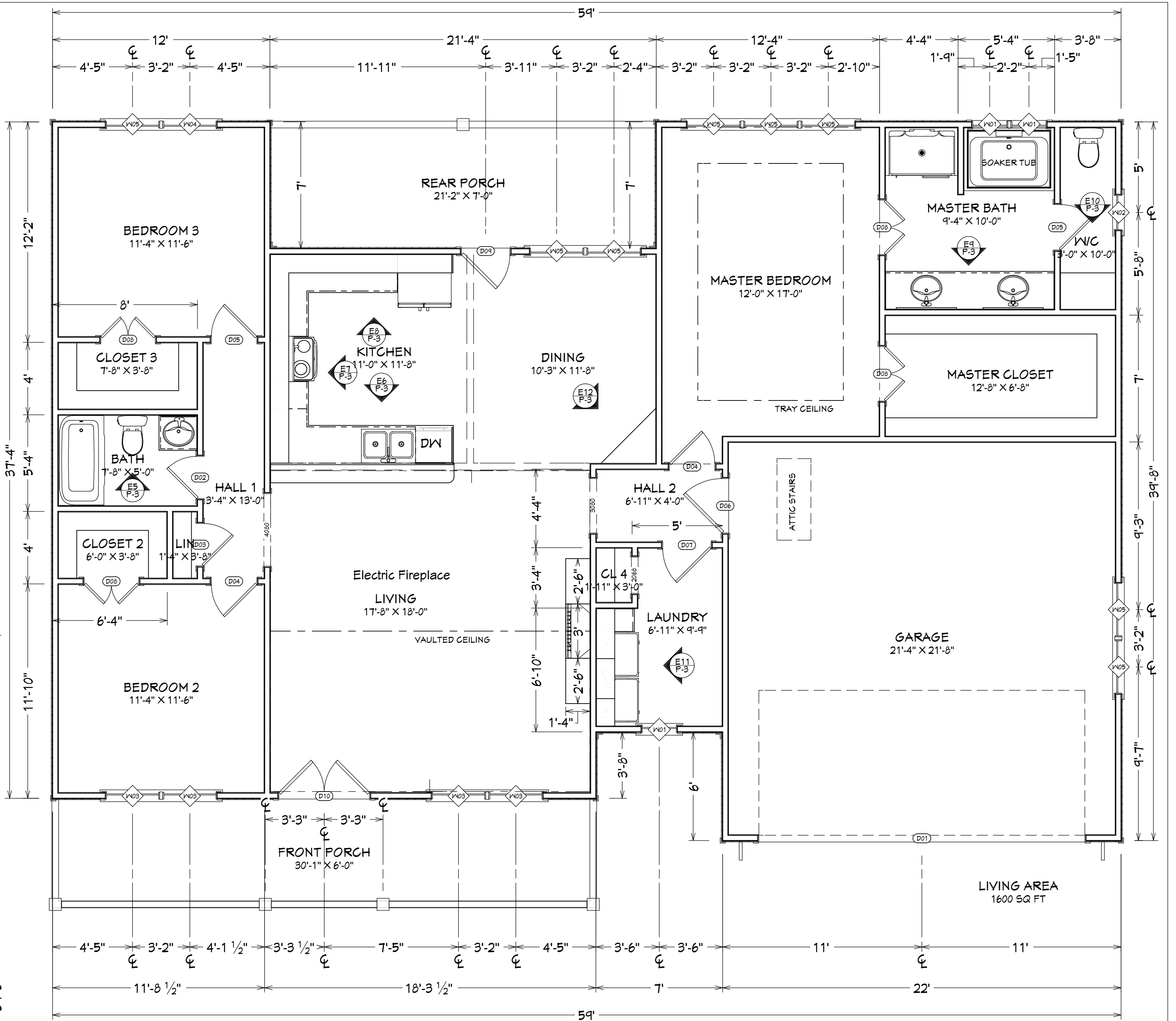
1ST FLOOR 1/4 IN = 1 FT
