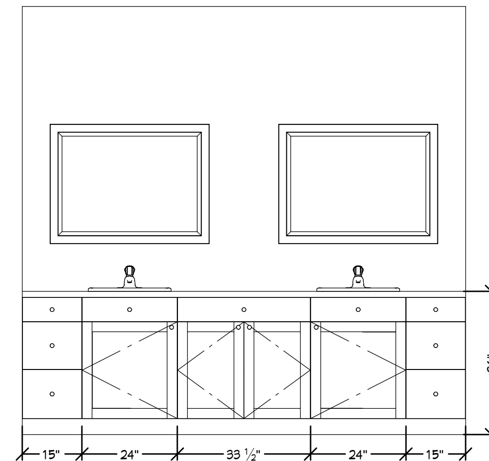
E9 ELEVATION 7 1/2 IN = 1 FT
