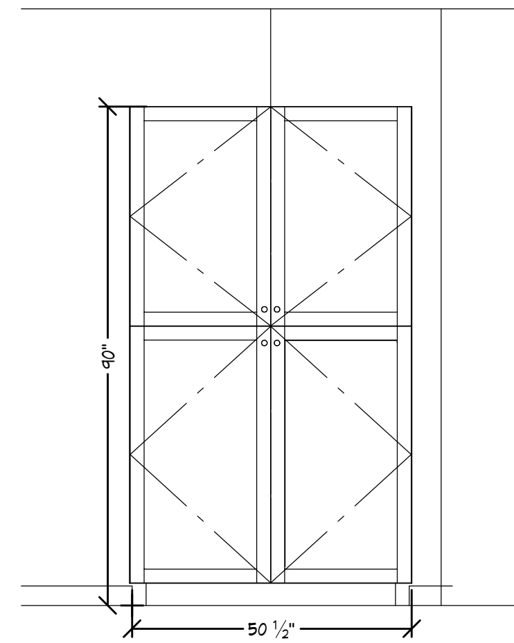
E12 ELEVATION 10 1/2 IN = 1 FT
