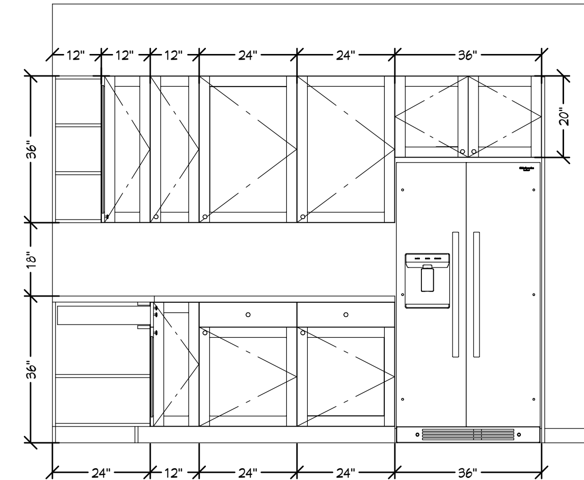
E8 ELEVATION 6 1/2 IN = 1 FT
