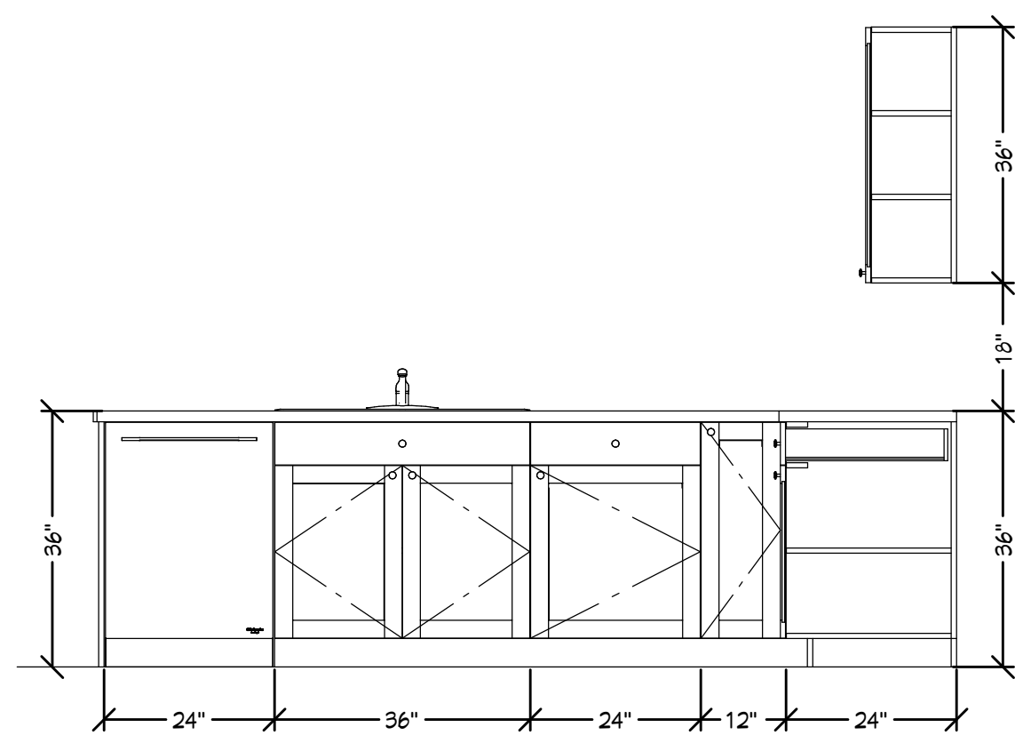
E6 ELEVATION 4 1/2 IN = 1 FT
