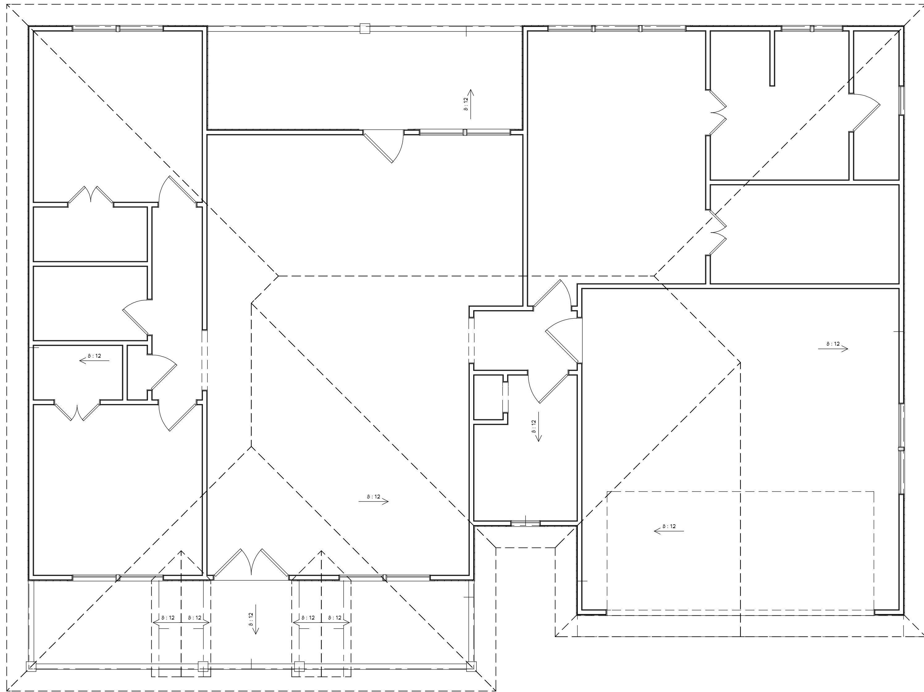
ROOF PLAN VIEW 1/4 IN = 1 FT
